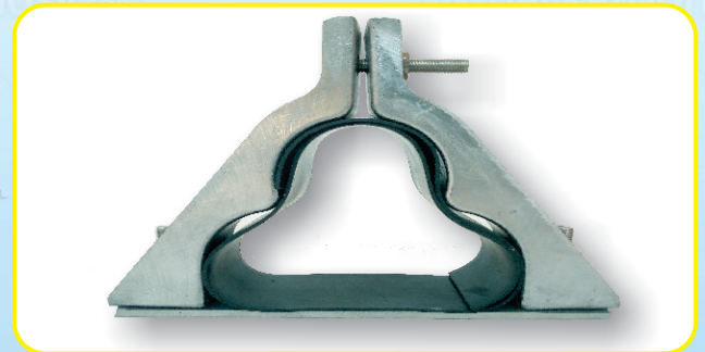
CLEAT FOR TREFOIL FORMATION
